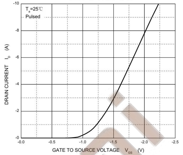
Transfer Characteristics
