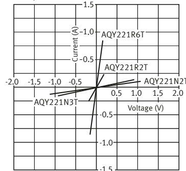
9-1. Current vs. voltage characteristics of output at MOS portion
