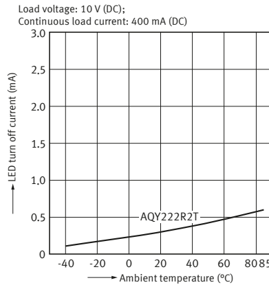
6-1. LED turn off current vs. ambient temperature characteristics
