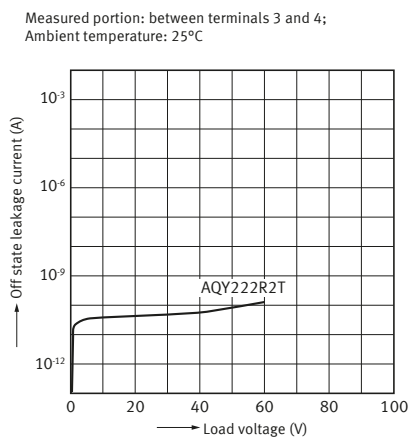
9-1. Off state leakage current vs. load voltage characteristics
