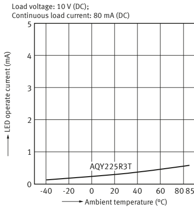
5-2. LED operate current vs. ambient temperature characteristics
