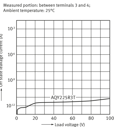
9-2. Off state leakage current vs. load voltage characteristics
