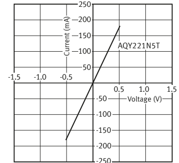
9-2. Current vs. voltage characteristics of output at MOS portion
