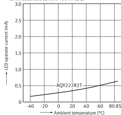
5-1. LED operate current vs. ambient temperature characteristics
