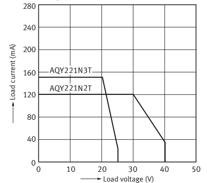
2-1. Load current vs. load voltage characteristics
