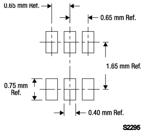
Figure 7. AS183-92LF-HX PCB Layout Footprint (Top View)
