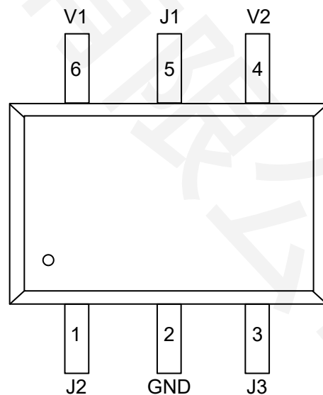
Figure 2. AS183-92LF-HX Pinout –6-Pin SC-70 (Top View)
