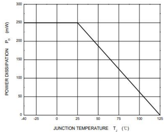
Figure 6: Power Characteristics
