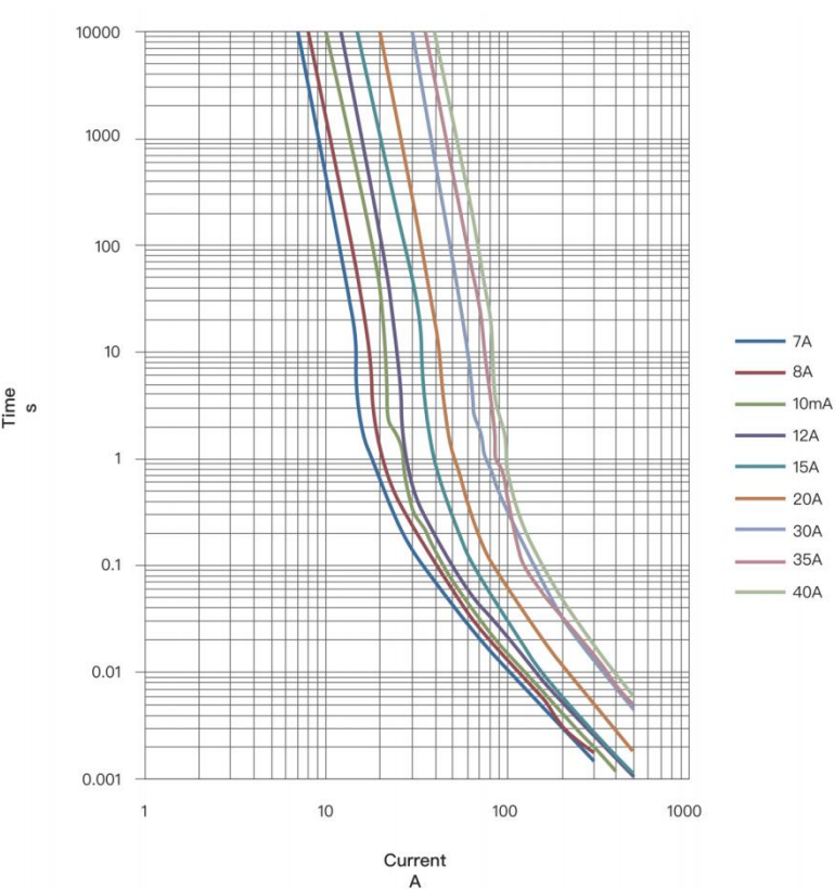
LTC2410TSK Series I-T Curve 7A~40A
