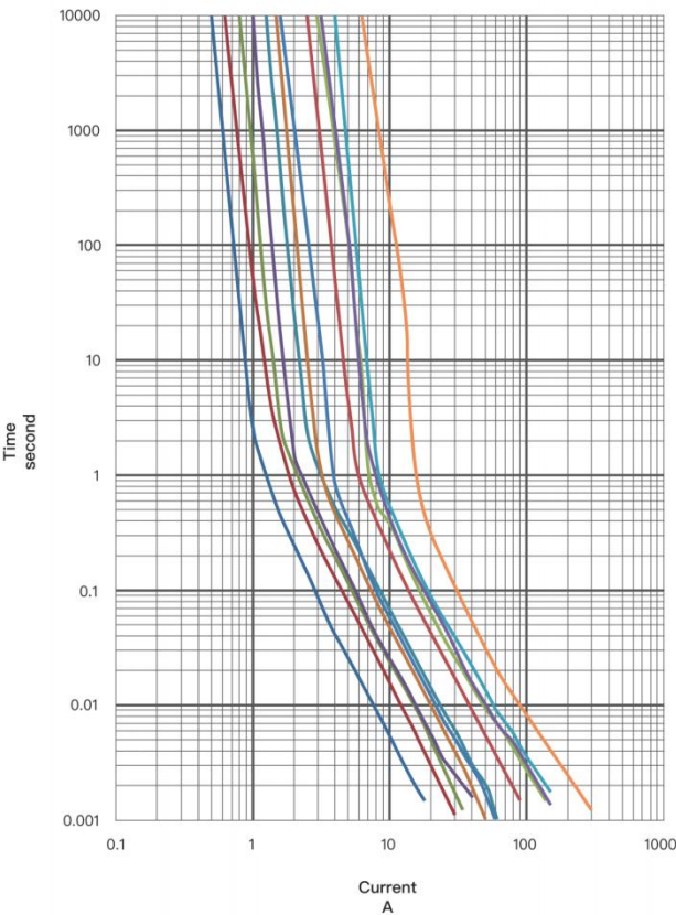
LTC2410TSK Series I-T Curve 500mA~6.3A
