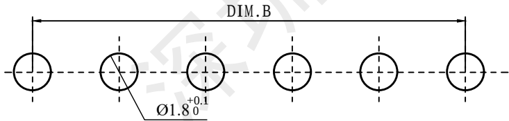
PCB LAYOUT
