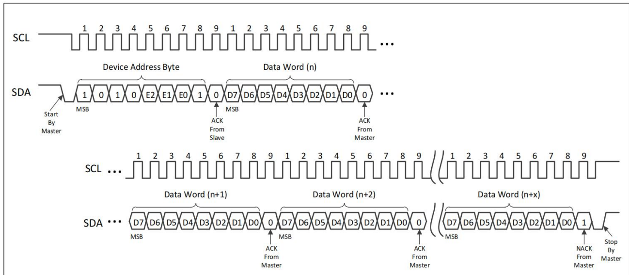
Figure 14 Sequential Read
