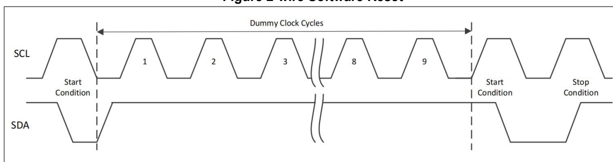
Figure 2-wire Software Reset
