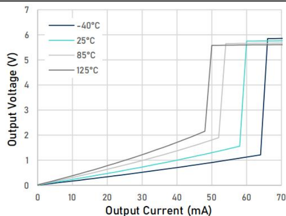
Output Voltage Swing as a function of Output Current (Sinking, V_S = 20\text{ V} )
