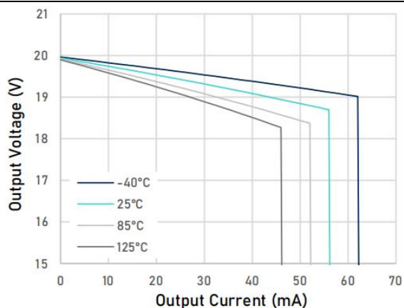
Output Voltage Swing as a function of Output Current (Sourcing, V_S = 20\text{ V} )
