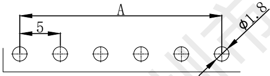
PCB LAYOUT
