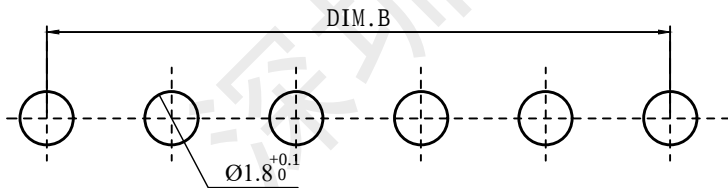
PCB LAYOUT
