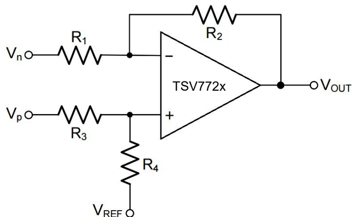
Figure 8. Differential Amplifier
