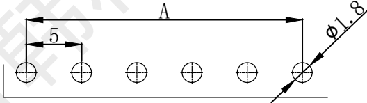
PCB LAYOUT
