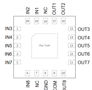
QFN-20 4*4
