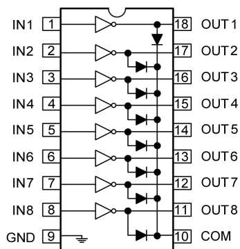
DIP-18/SOP-18
