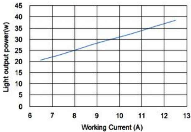
Light output power vs. current
