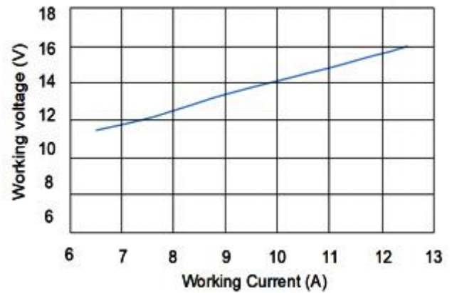
Working voltage vs. Working Current
