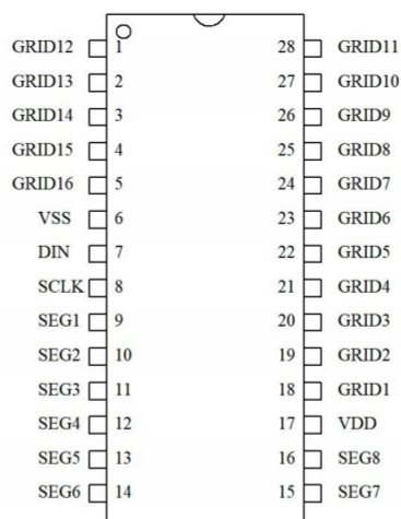
GM1640 28SOP/SSOP
