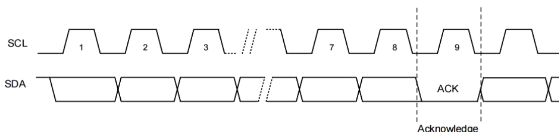
Figure 4-3 Output Acknowledge
