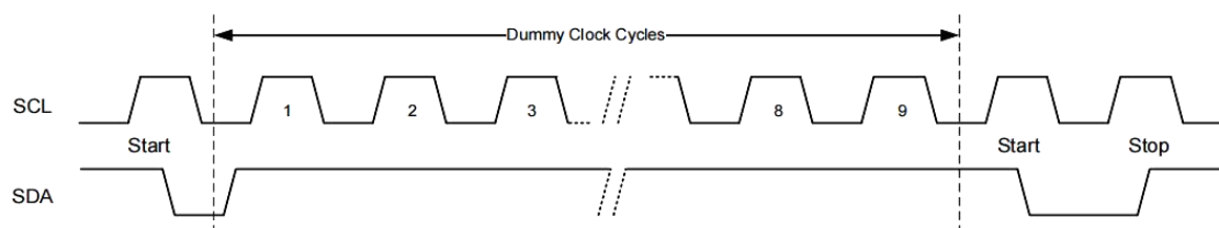
Figure 4-4 Soft Reset
