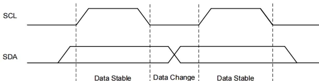
Figure 4-1 Data Validity
