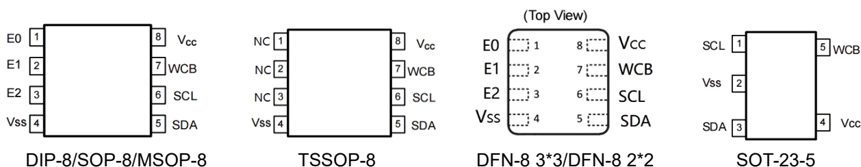
Figure 1-1 Pin Configuration
