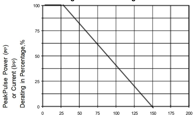
Fig.2 - Pulse Derating Curve
