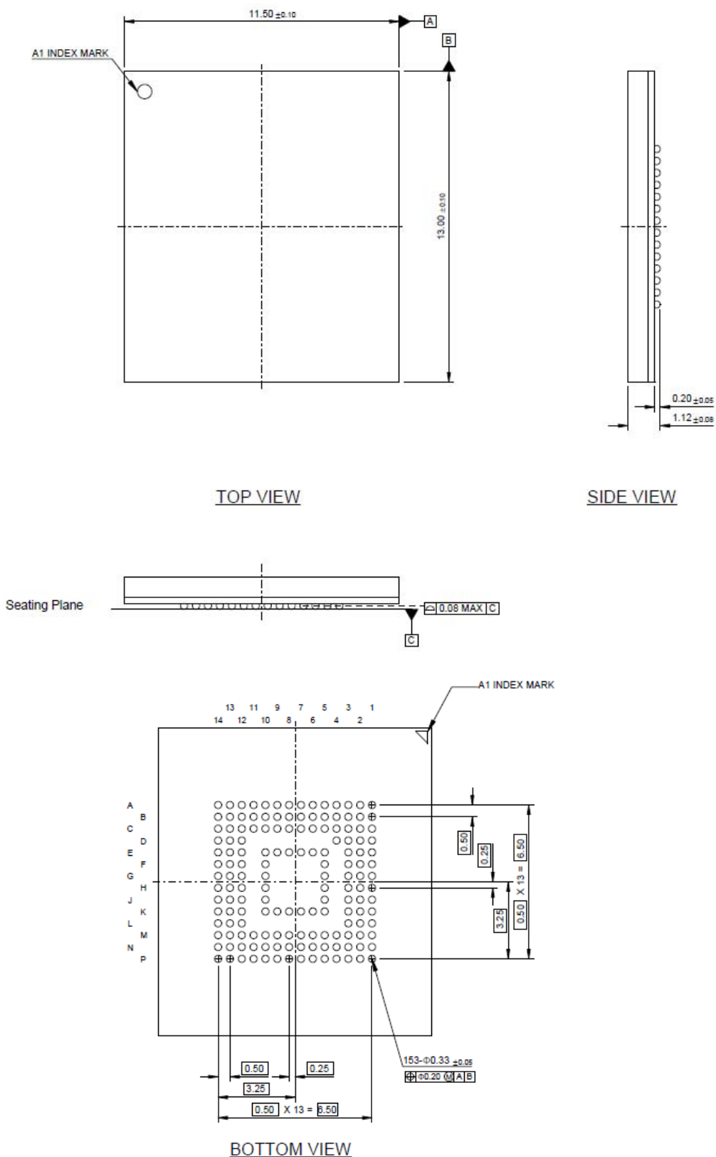
Figure 2. 11.5mm x 13mm x 1.2mm Package Dimension
