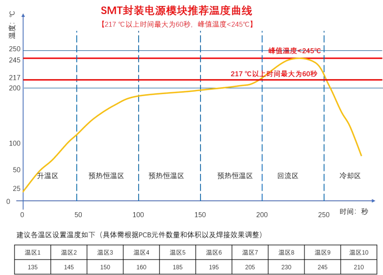
图 4：建议回流焊温度曲线 Figure 4: Suggested reflow soldering temperature curve
