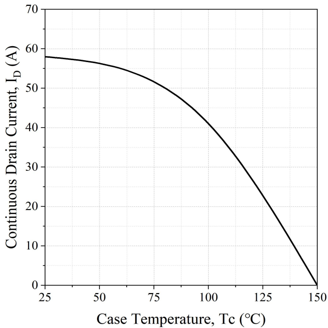
Fig 17. Current De-rating
