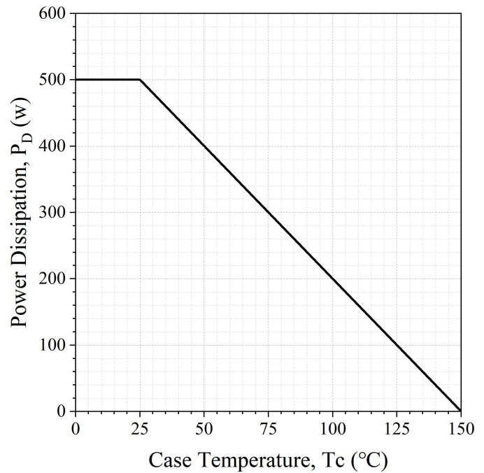
Fig 18. Power Dissipation De-rating
