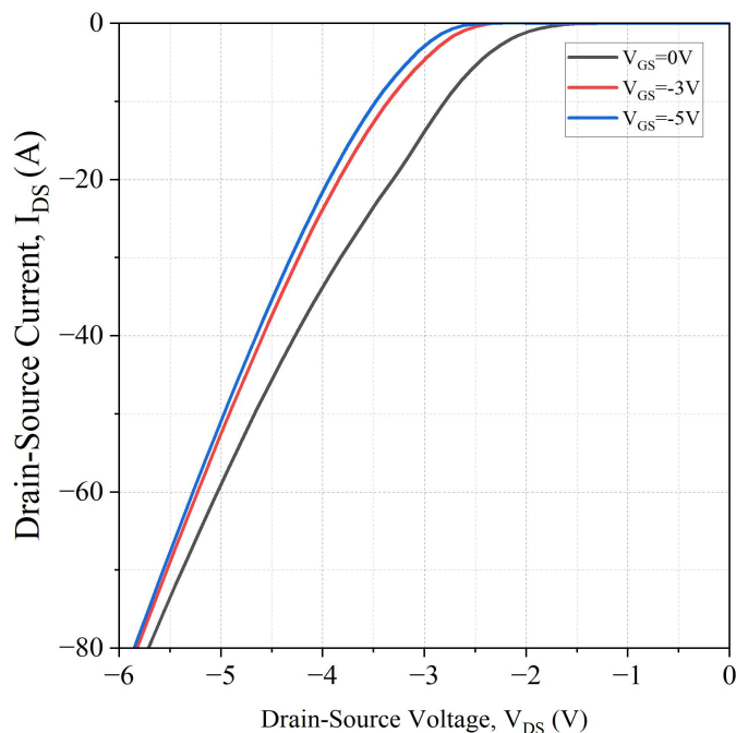
Fig 13. Body Diode Characteristics at Tj= 25°C
