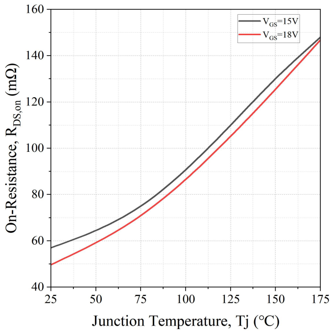
Fig 5. On-Resistance vs. Temperature
