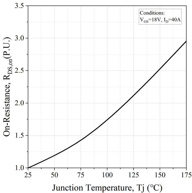
Fig 7. Normalized On-Resistance vs. Temperature
