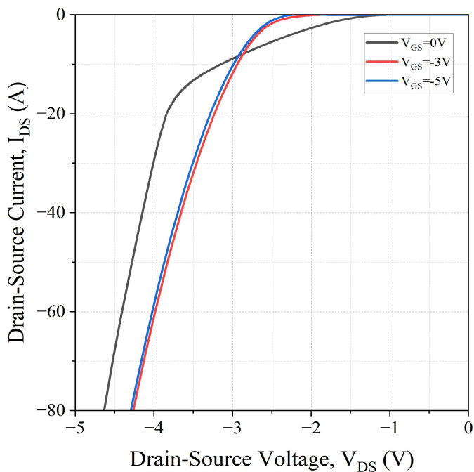
Fig 14. Body Diode Characteristics at Tj= 175°C
