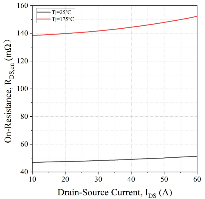
Fig 6. On-Resistance vs. Drain current
