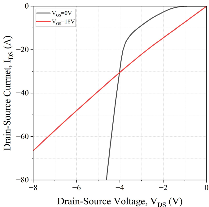
Fig 16. 3rd Quadrant Characteristic at Tj= 175°C
