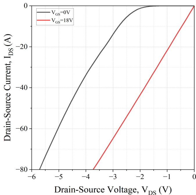
Fig 15. 3rd Quadrant Characteristic at Tj= 25°C
