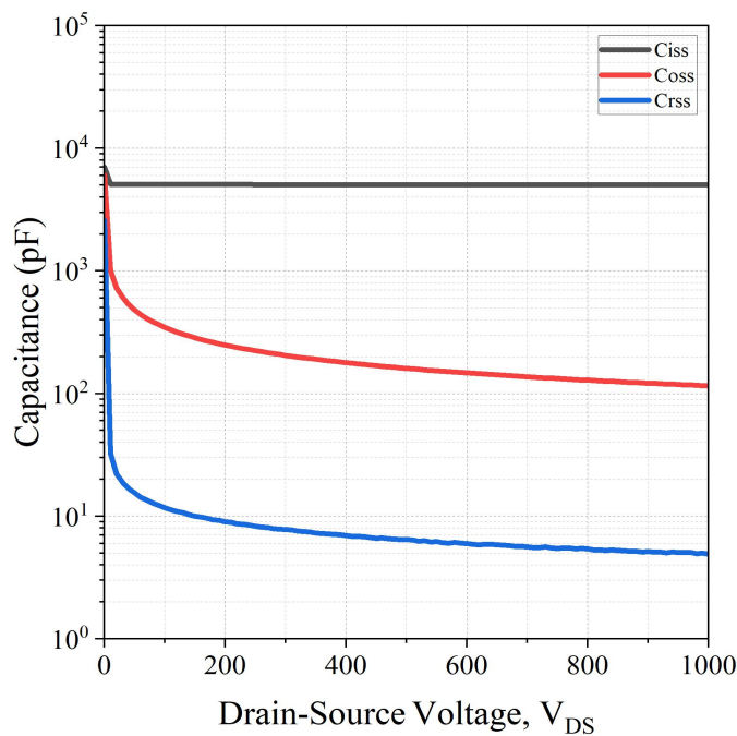
Fig 11. Capacitances vs. Drain-Source
