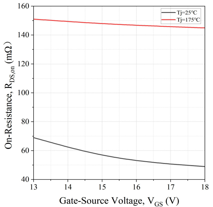
Fig 8. On-Resistance vs. Gate Voltage
