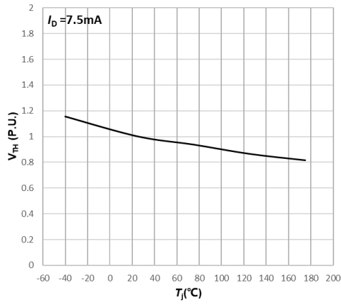
Fig7. Normalized Threshold Voltage vs. Temperature For T_j = 25^\circ\text{C}
