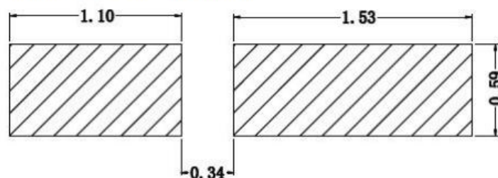
建议焊盘尺寸图 Recommended Soldering Pattern
