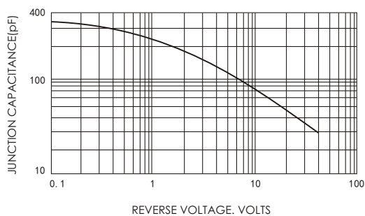
FIG.5-TYPICAL JUNCTION CAPACITANCE
