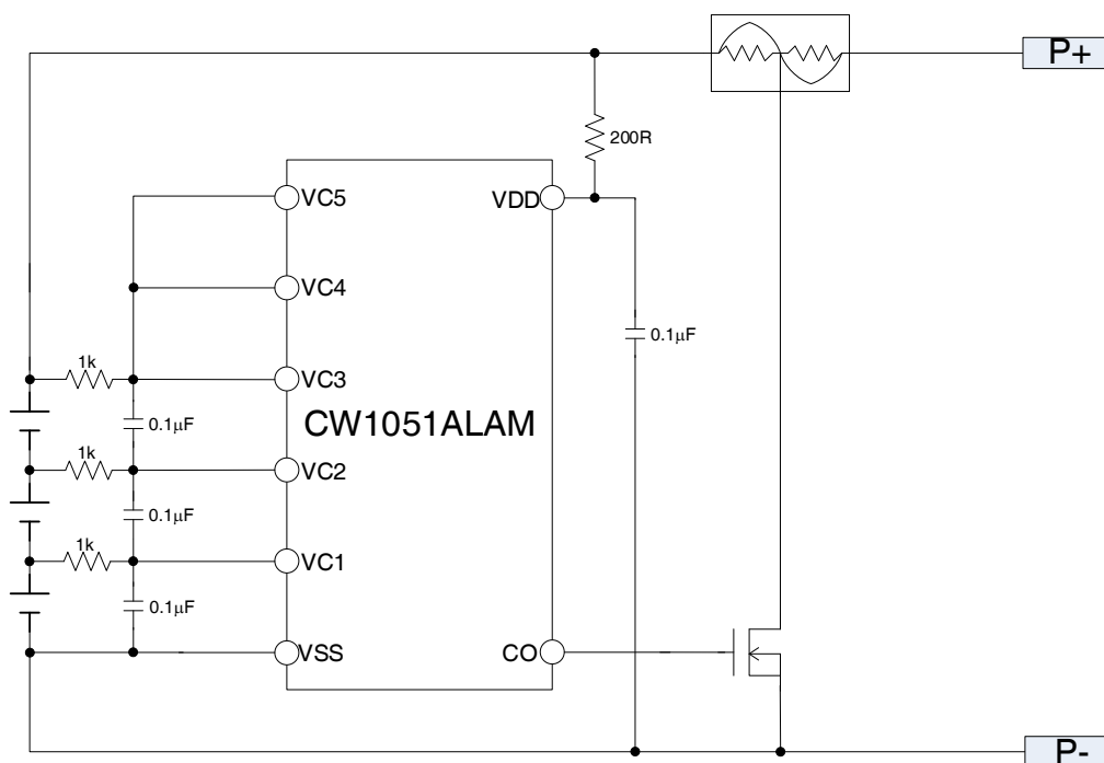
Reference Schematic for 3 cells(connect high side cell)
