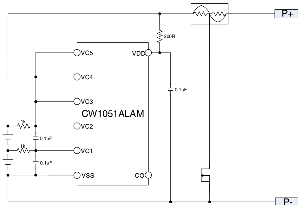
Reference Schematic for 2 cells(connect high side cell)
