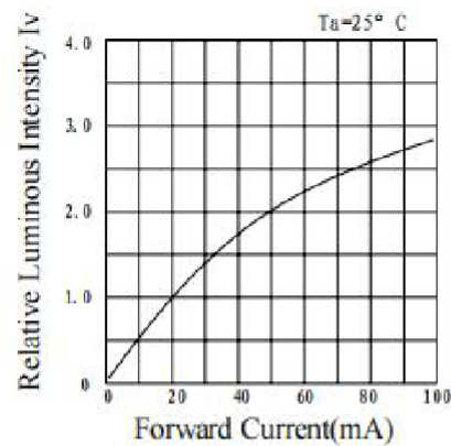
b) 相对光强—正向电流 b) RELATIVE LUMINOUS INTENSITY VS. FORWARD CURRENT
