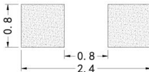
Recommend Pad Layout
