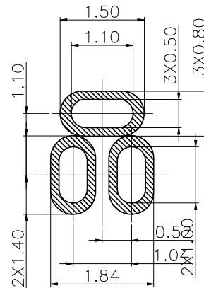
RECOMMENDED PCB LAYOUT TOLERANCE±0.05(焊盘推荐图) (FOR REFERENCE ONLY)
