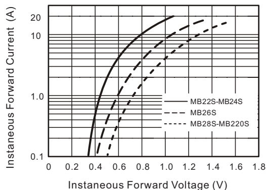
FIG.2-TYPICAL FORWARD CHARACTERISTICS
