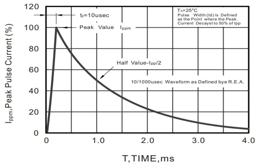
Fig.3 Pulse Waveform
