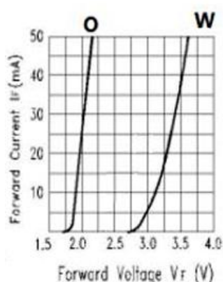
Fig.2 Forward Current vs. Forward Voltage
