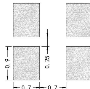
Recommended Soldering Pad
