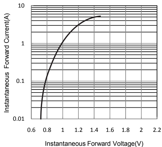
FIG.2-TYPICAL FORWARD CHARACTERISTICS
