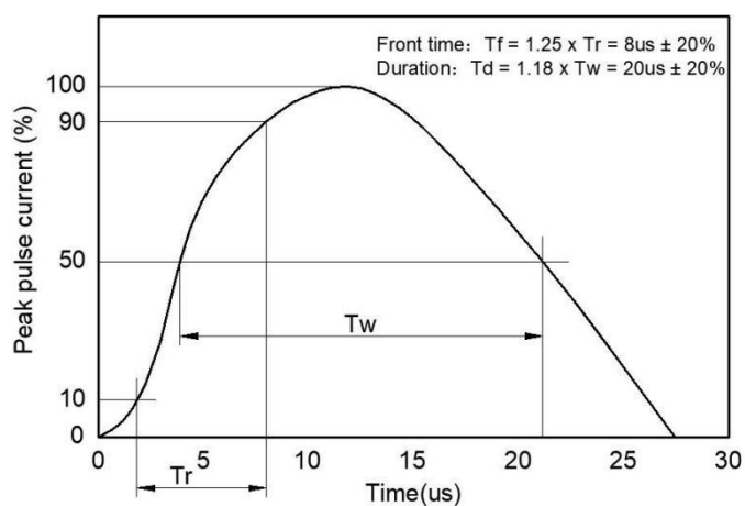
FIG2: pulse Waveform
