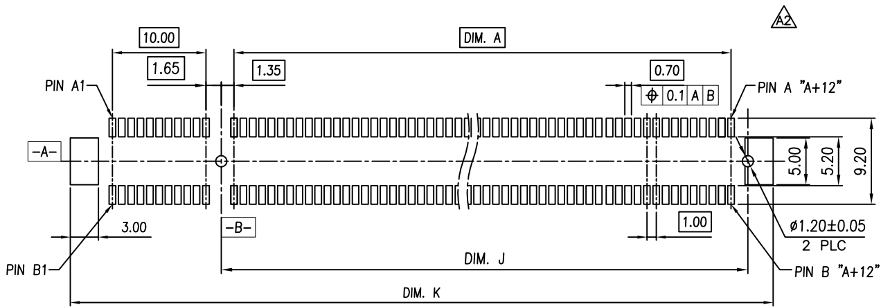
RECOMMENDED PCB LAYOUT (COMPONENT SIDE) TOLERANCE: \pm 0.05
