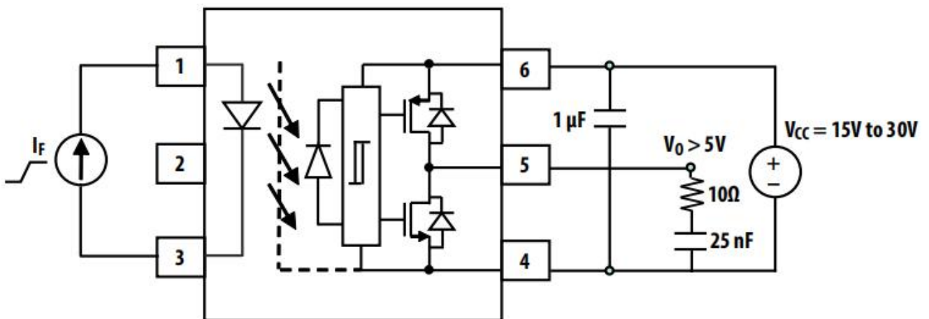
Figure.16 I_{FH} Test Circuit
