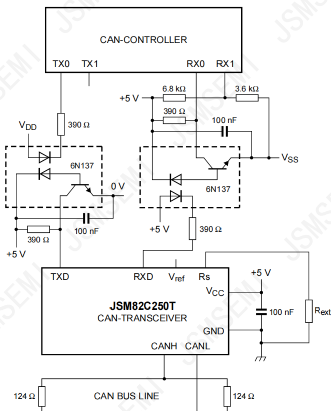
Figure 8.Application with galvanic isolation.
