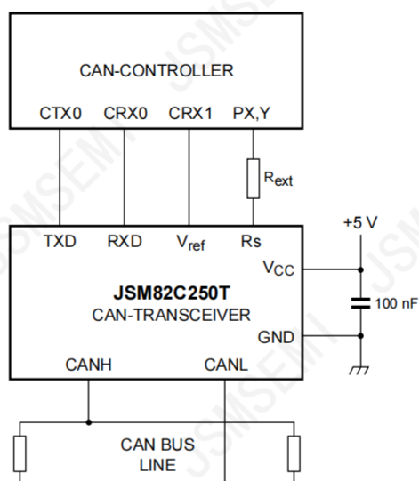
Figure 7.Application of the CAN transceiver.
