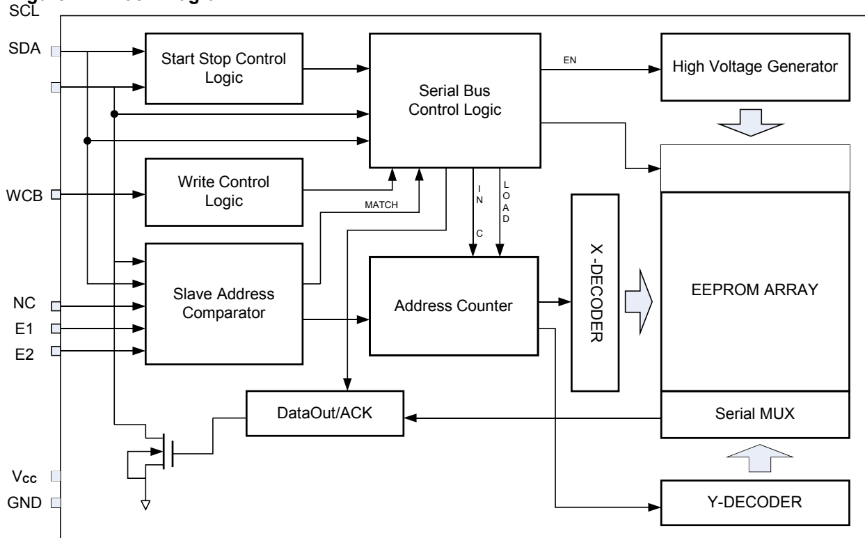
Figure 2-1 Block Diagram
