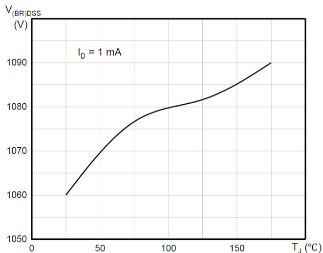
Figure 13. Breakdown Voltage vs. Temperature
