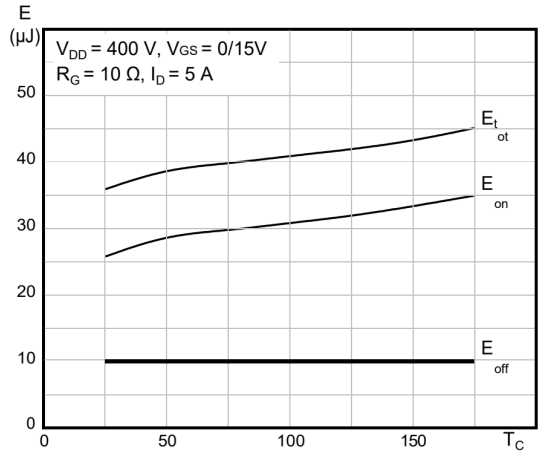
Figure 12. Typical Switching Energy vs. Temperature
