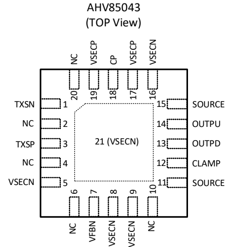
Pinout Table [1]
