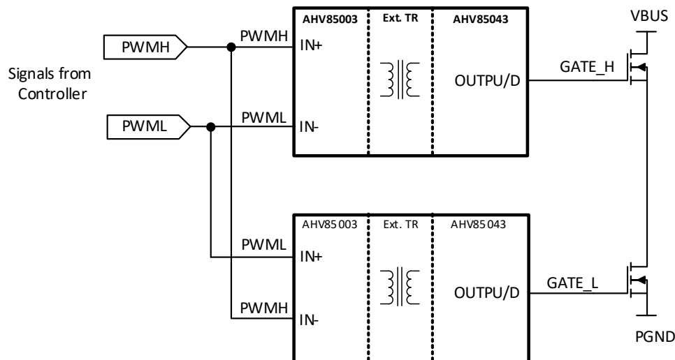
Figure 8: Interlock Connection of PWML and PWMH to IN+ and IN- In Half-Bridge Leg for Shoot-Through Protection,
