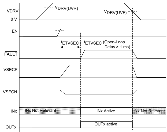
Figure 3: Startup Time and Sequence, and V_{DRV} Supply UVLO, AHV85003 and AHV85043 Chipset with Recommended External Transformer
