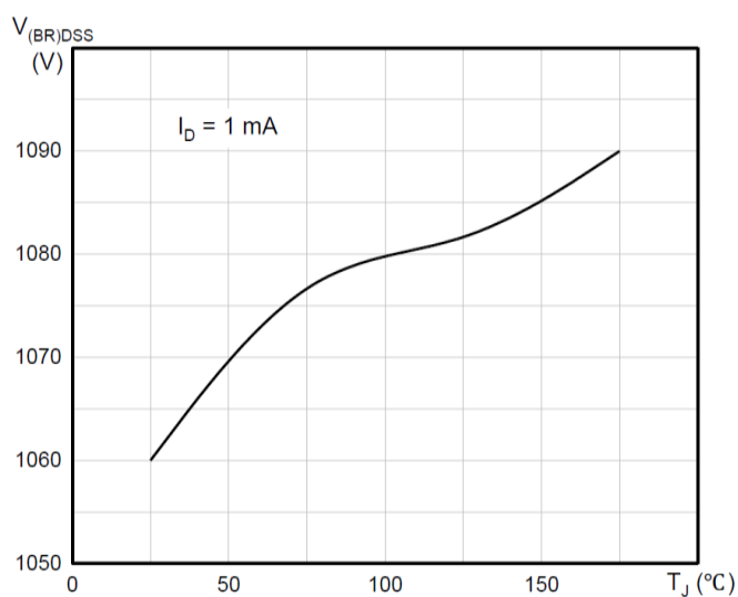
Figure 13. Breakdown Voltage vs. Temperature
