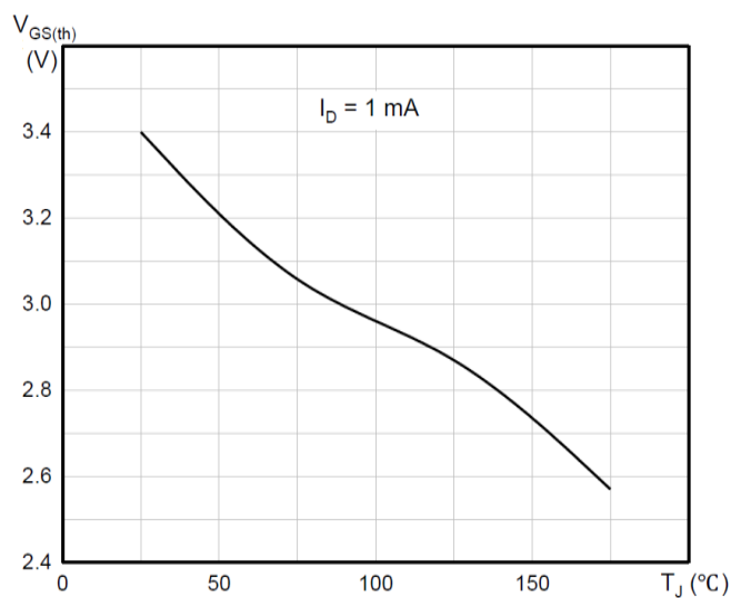
Figure 14. Gate Threshold vs. Temperature
