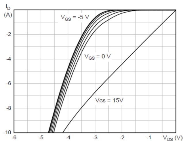
Figure 17. Body Diode Characteristics, T_j = 175^\circ\text{C}
