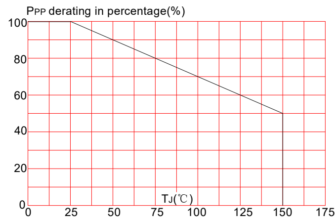
FIG.5: Pulse derating curve (10/1000µs)
