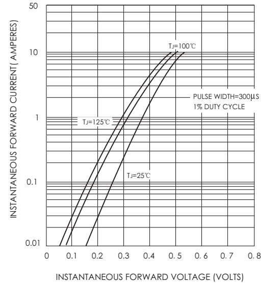
FIG.2-TYPICAL FORWARD CHARACTERISTICS
