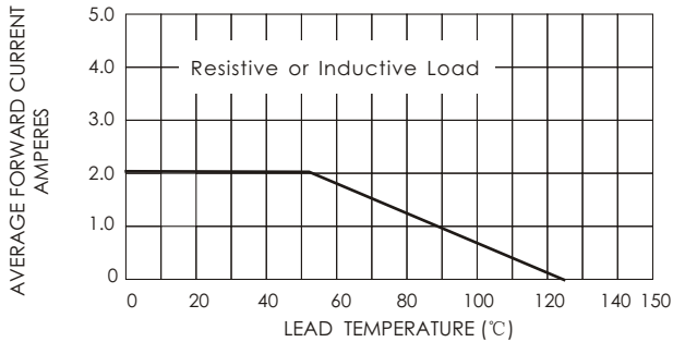
FIG.1-TYPICAL FORWARD CURRENT DERATING CURVE
