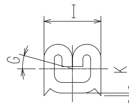
WIRE BARREL CROSS-SECTION IMAGE
