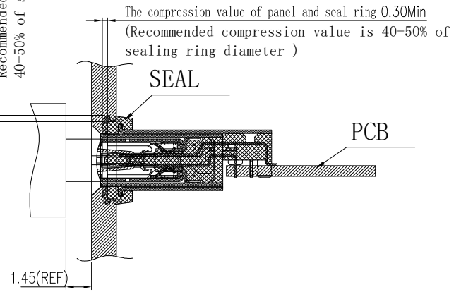
Schematic drawing after mating
