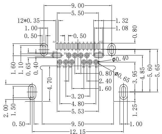
RECOMMENDED PCB LAYOUT, TOP VIEW (THICKNESS=0.60MM; TOLERANCE: \pm 0.05 )
