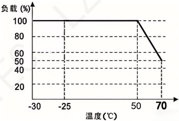
TEMPERATURE VS. LOAD
