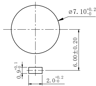
Panel layout
