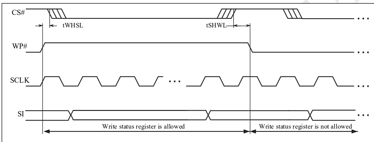
Figure 5-7 WP Timing
