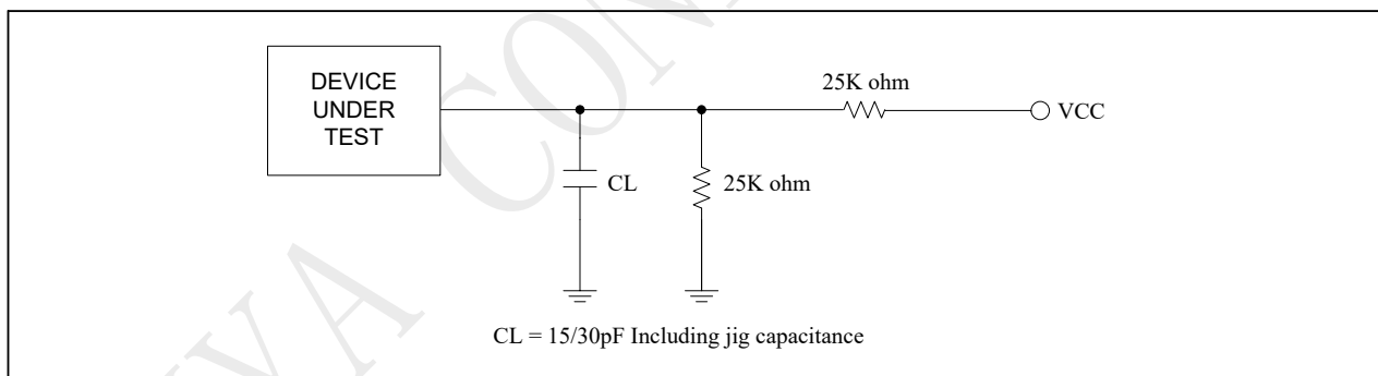
Figure 5-2 Output Loading
