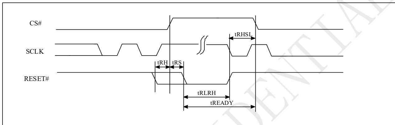
Figure 10-51 RESET Timing
