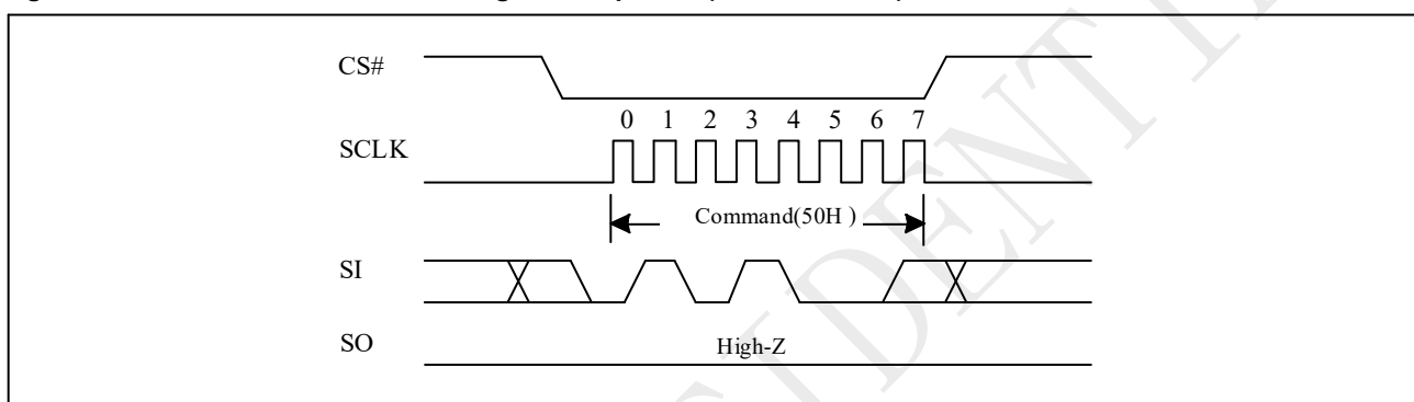
Figure 10-4 Write Enable for Volatile Register Sequence (Command 50h)
