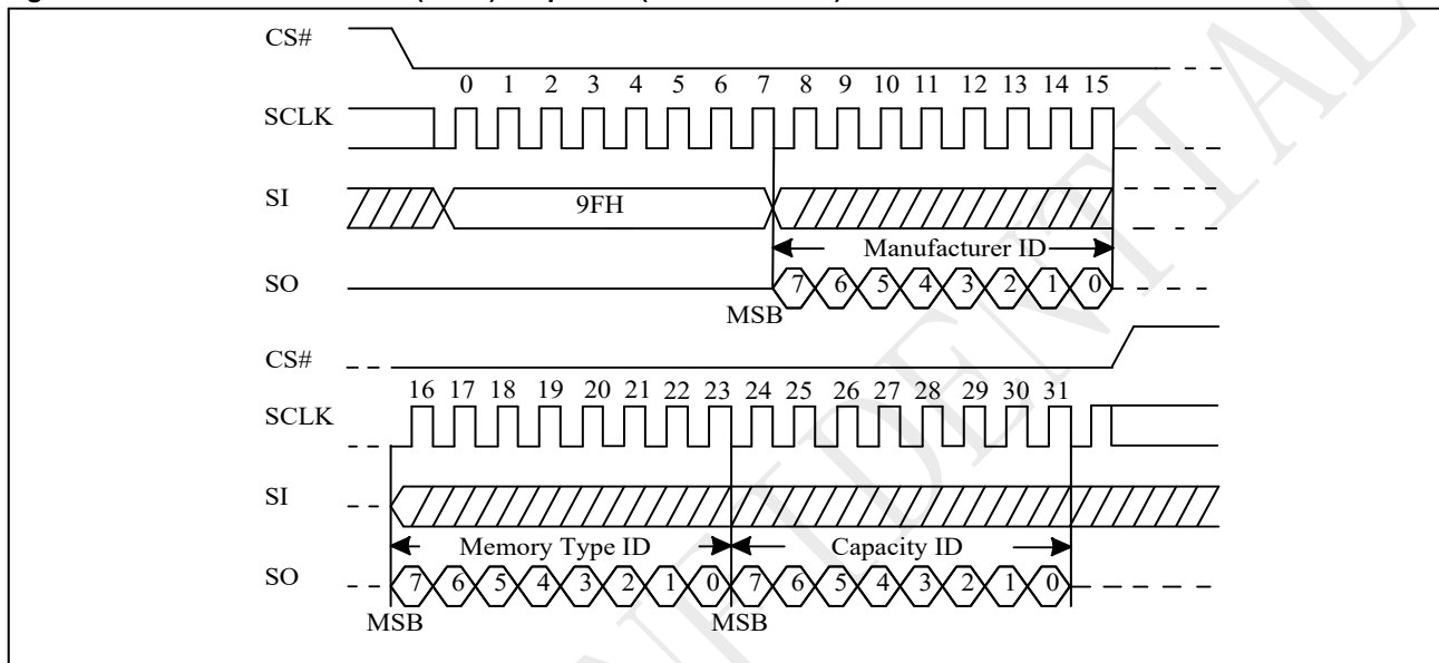
Figure 10-40a Read Identification (RDID) Sequence (QPI)
