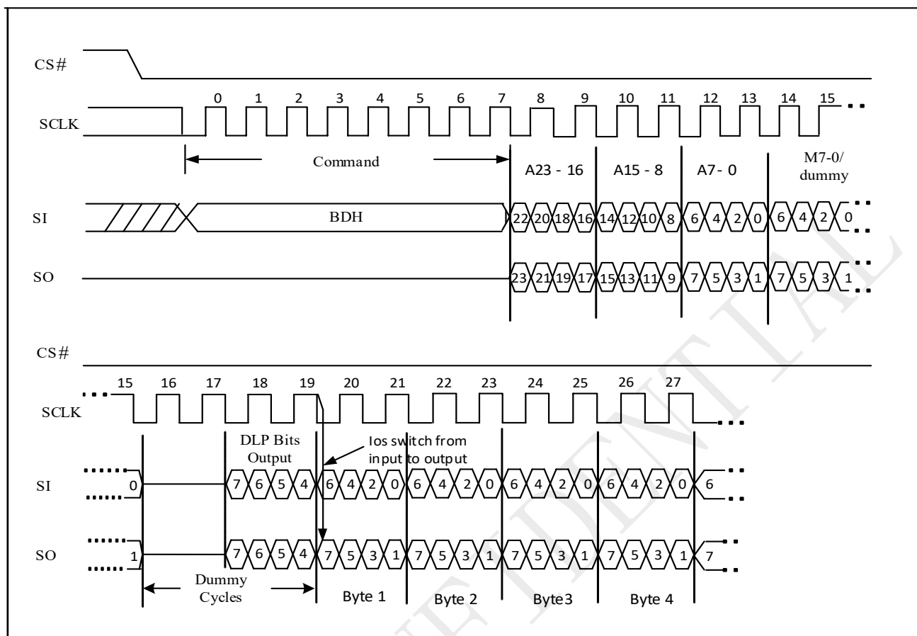
Figure 10-23l DTR 4IO Read with DLP bits output Sequence
