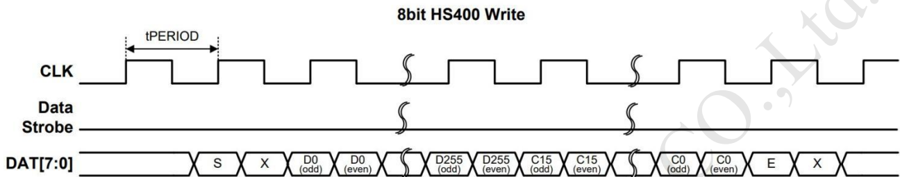
Figure.6 HS400 Write Timing with data block size of 512 bytes
