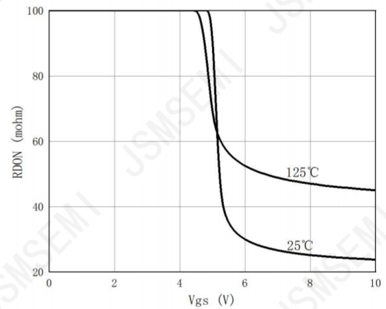
Figure 10: On-Resistance vs. Gate-Source Voltage
