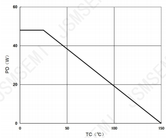
Figure 12: Power De-rating
