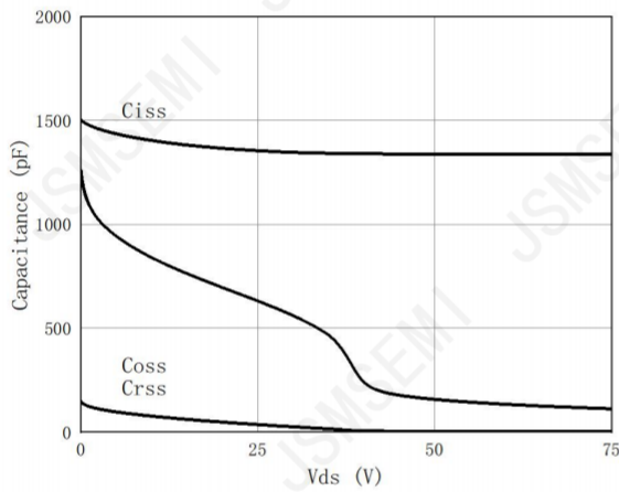
Figure 9: Capacitance
