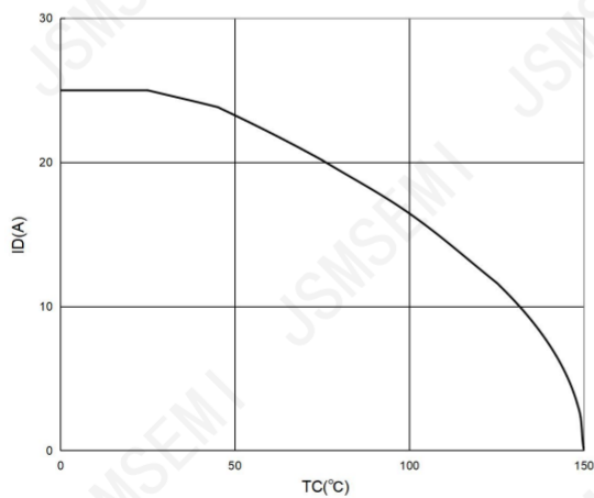
Figure 11: Current De-rating
