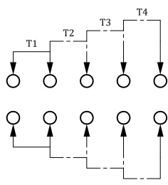
SCHEMATIC(SHORTING)
